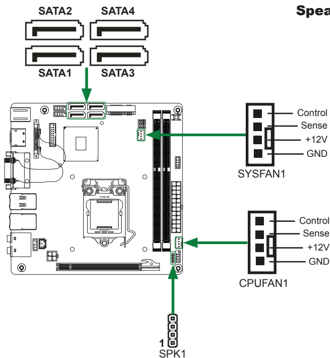
SPK1-Pin Definition
