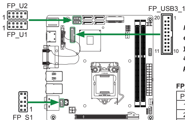
FP_U1~FP_U2-Pin Definition
